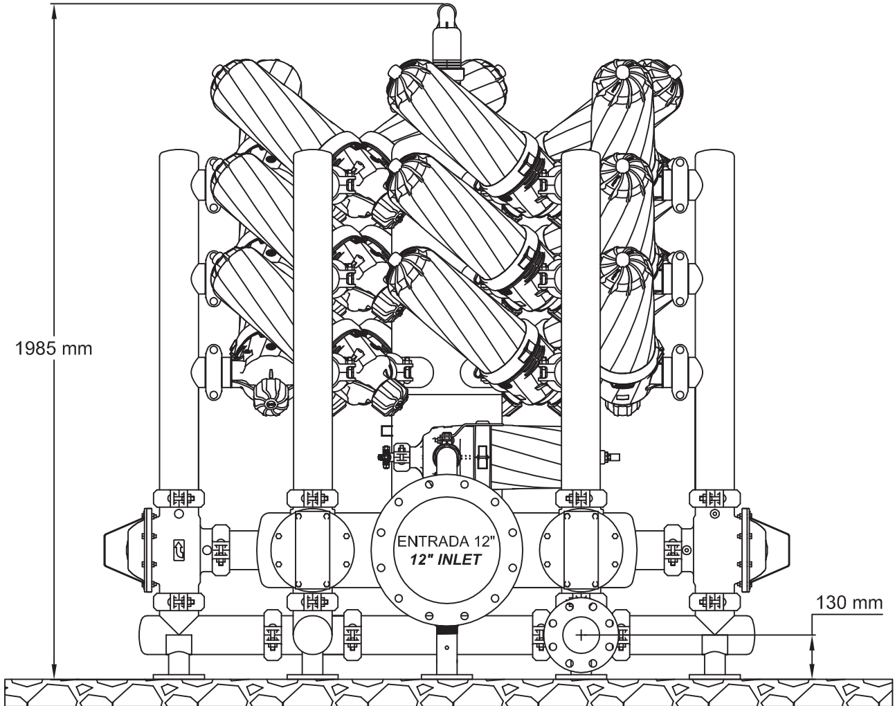
COLECTOR DRENAJE 4" 4" DRAINAGE MANIFOLD
